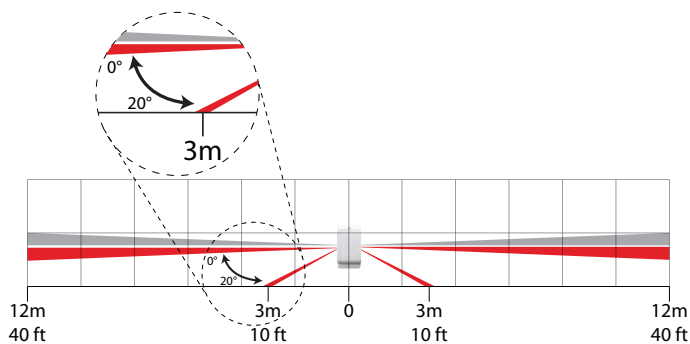
Figure 1: Range Adjustment
